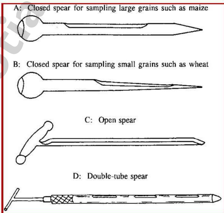
Simple bag sampling spears and D: Double tube spear
